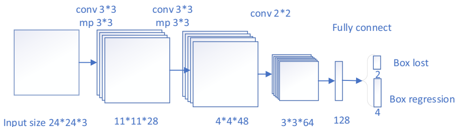
Fig. 3 FTNet Architecture
